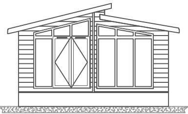
Elevation C
