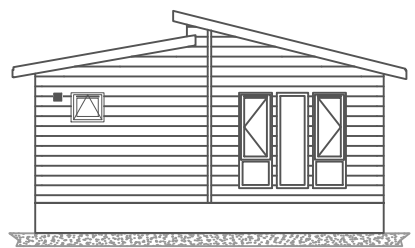
Elevation D
